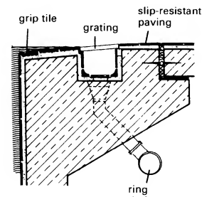
⑤ Finnish type rim and channel
